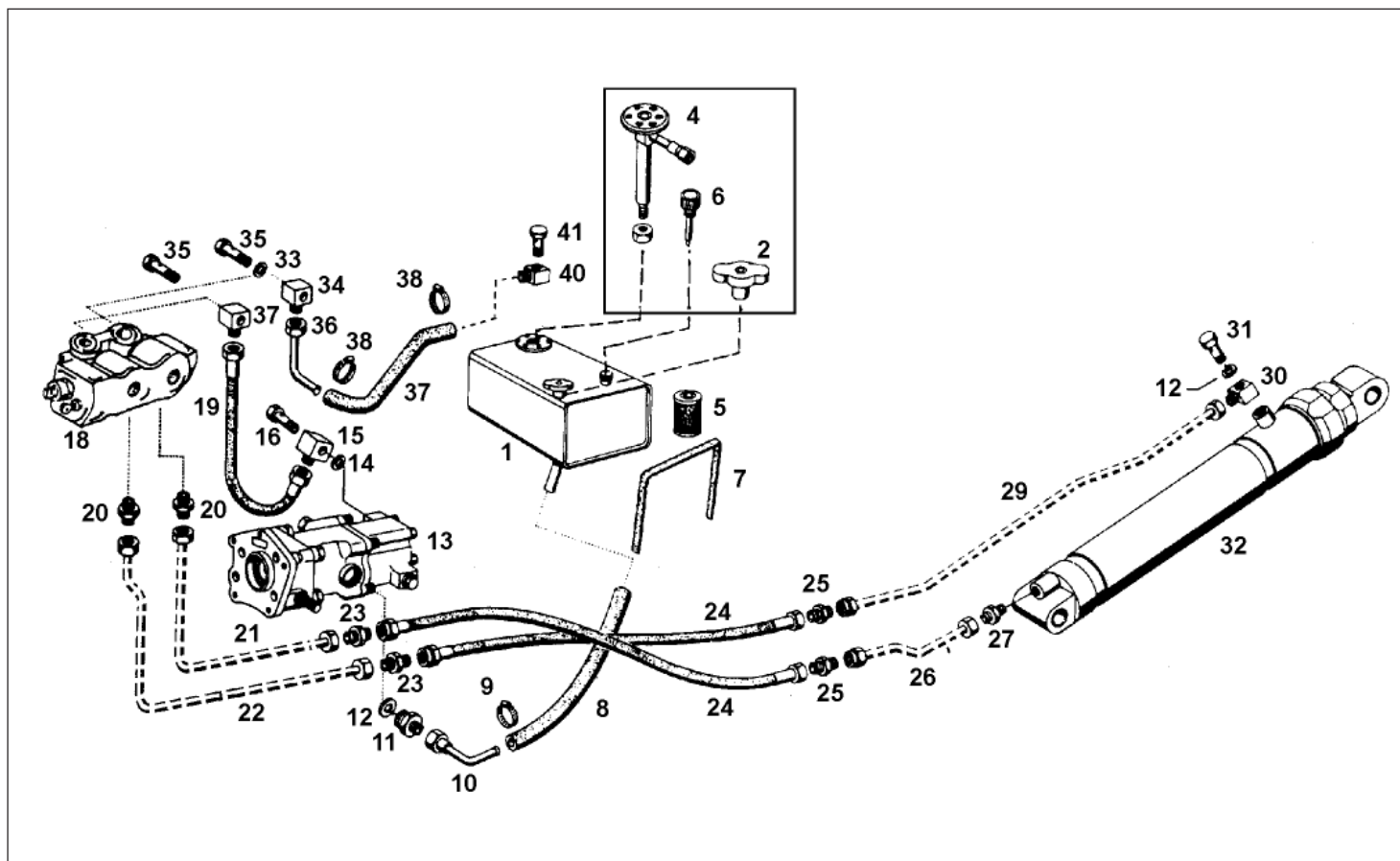
HYDRAULIC PIPE LINES (SINGLE TIPPER CYLINDER)
