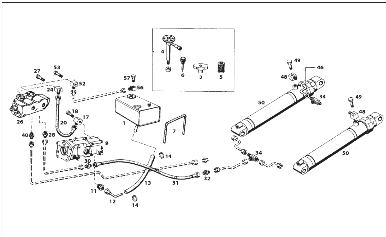
HYDRAULIC PIPE LINES (TWIN TIPPER CYLINDER)
