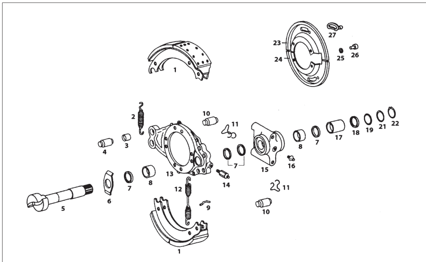
REAR WHEEL BRAKE (S-CAM) (AAL)
