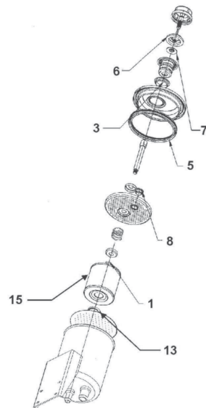
POWER STEERING HYDRAULIC TANK (CHINA)
