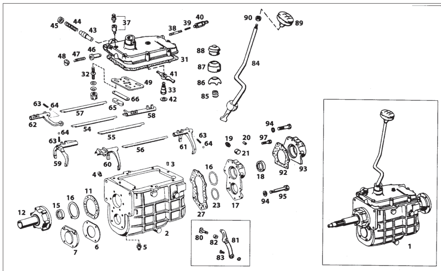
GEAR BOX, HOUSING AND COVER
